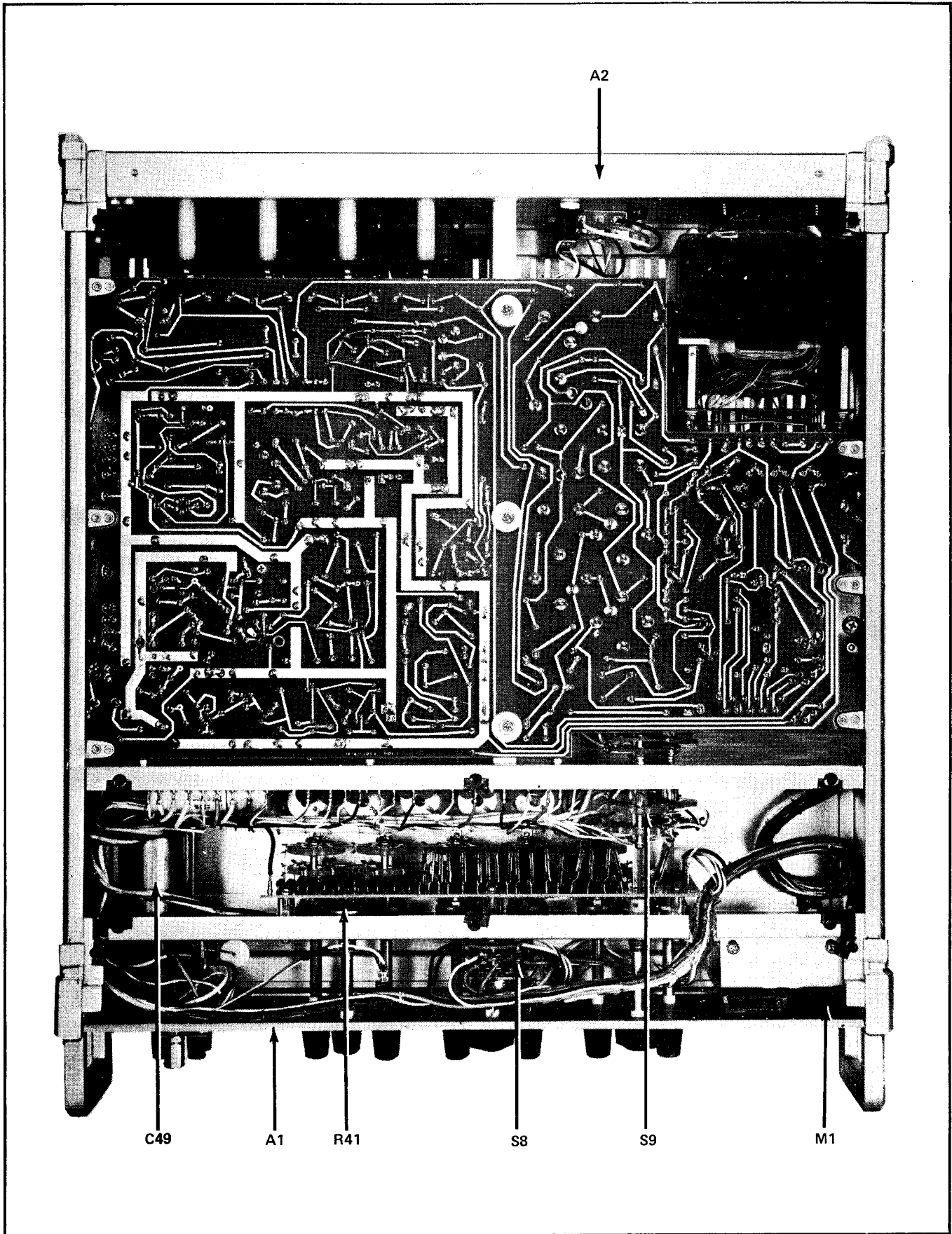
Figure 5-1. 341A DC VOLTAGE CALIBRATOR (Sheet 1 of 2)
