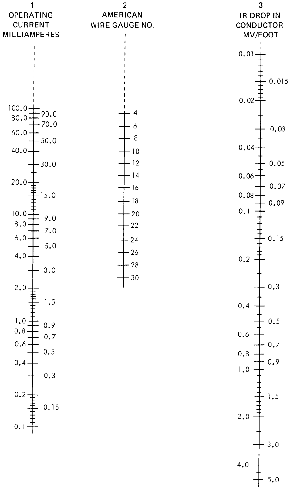
Figure 2-2. NOMOGRAPH OF VOLTAGE DROP IN LOAD WIRES
