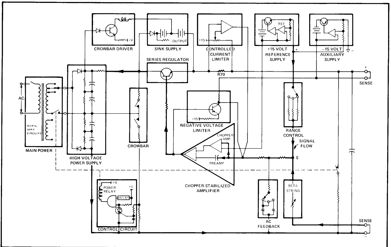
Figure 3-1. MODEL 341A/343A BLOCK DIAGRAM
