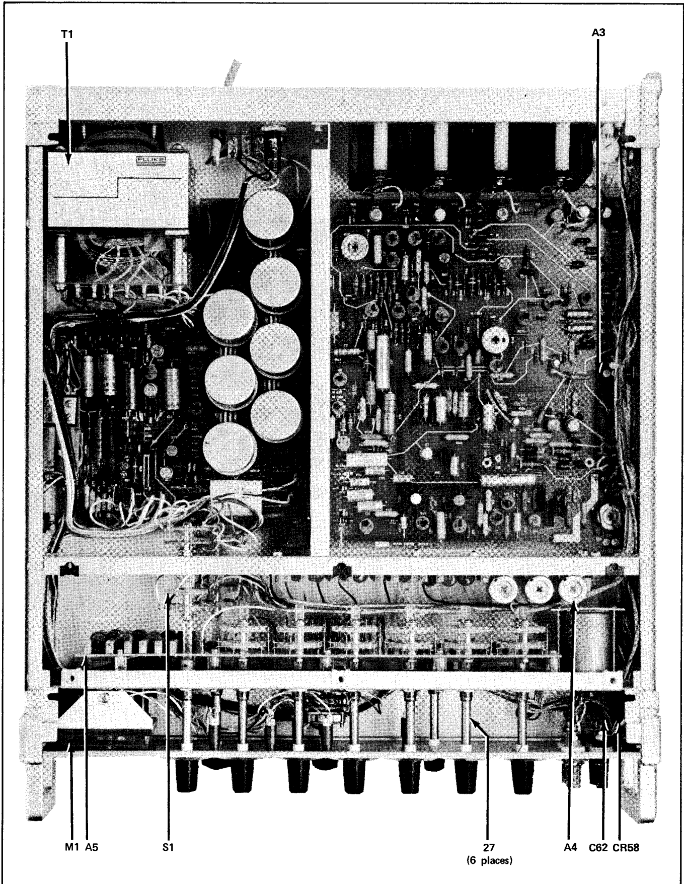
Figure 5-8. 343A DC VOLTAGE CALIBRATOR (Sheet 2 of 2)
