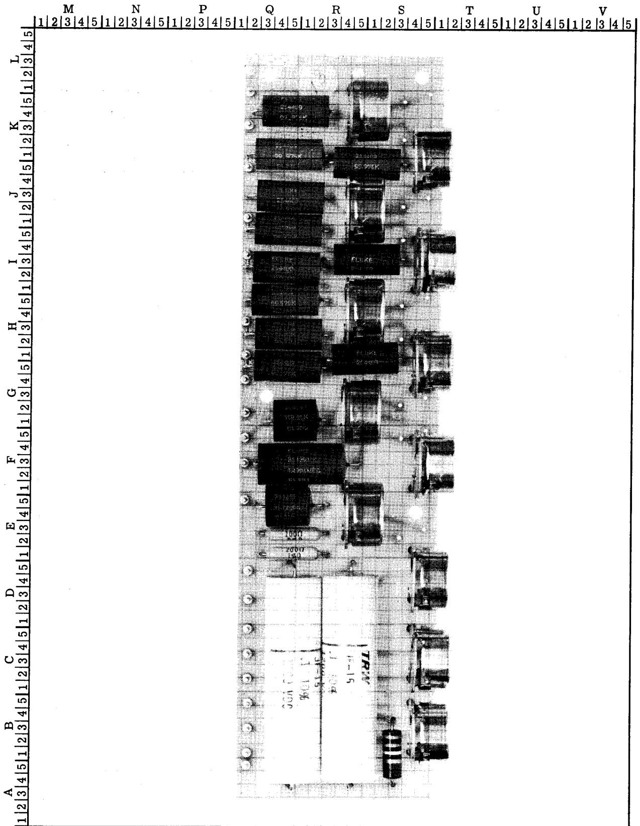
Figure 5-6. REFERENCE P/C ASSEMBLY (341A)
