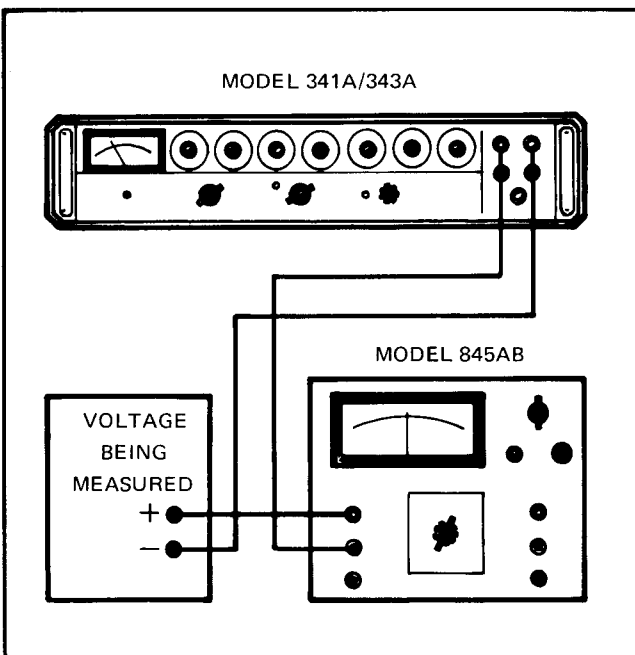
Figure 2-3. DIFFERENTIAL VOLTMETER
